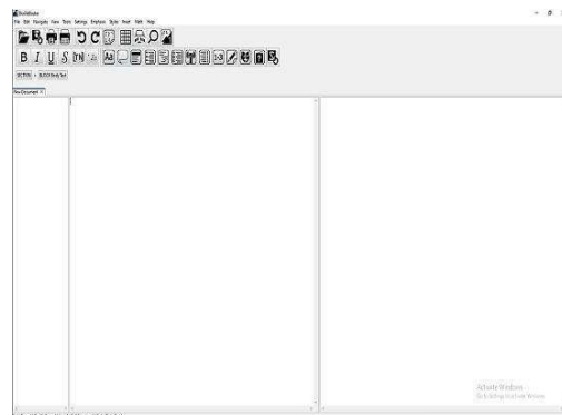
Braille-Blaster Software
