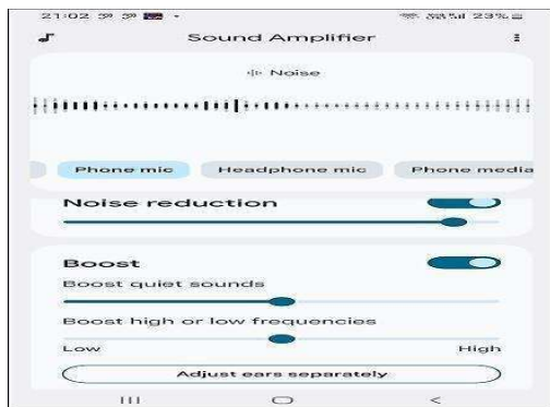
Sound-Amplifier Software
