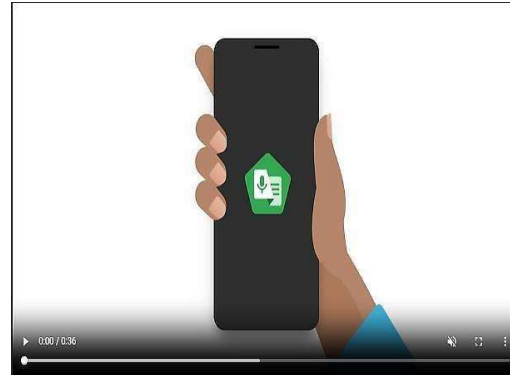
Live-Transcribe Software
